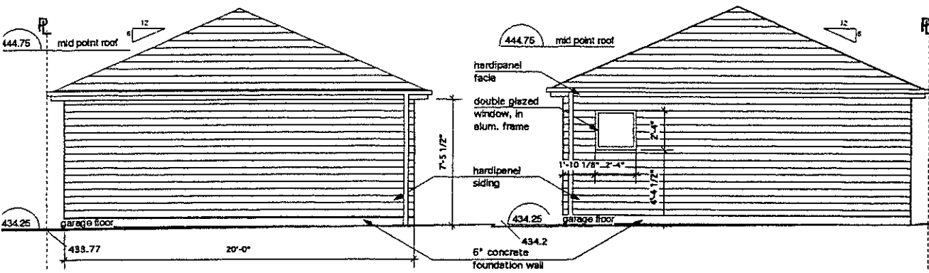
EAST ELEVATION
