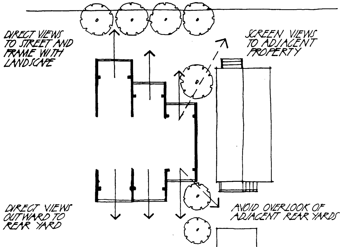
Figure 3. Examples of Building Configuration to ensure Privacy.
