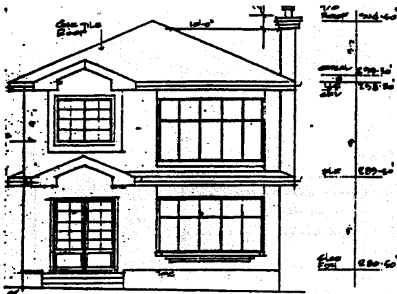
FRONT ELEVATION (W) LOT 6
