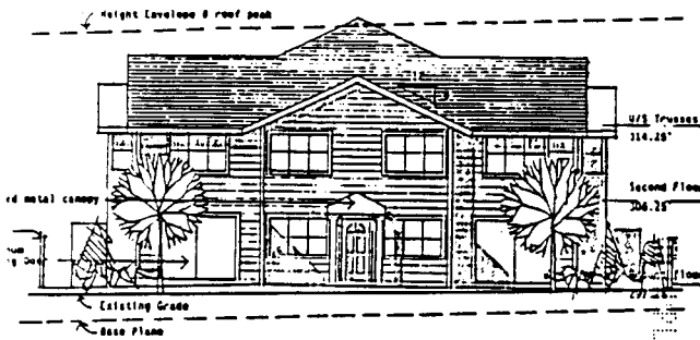
SOUTH ELEVATION / E. 28th AVENUE Scale: 1/8"=1'-0"
